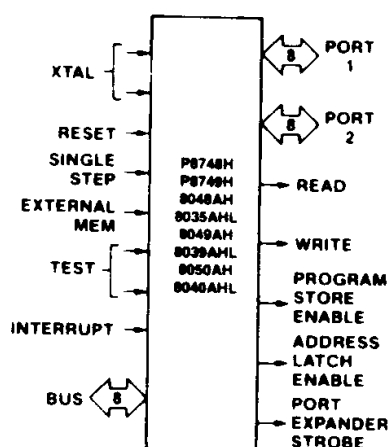
Figure 2. Logic Symbol
