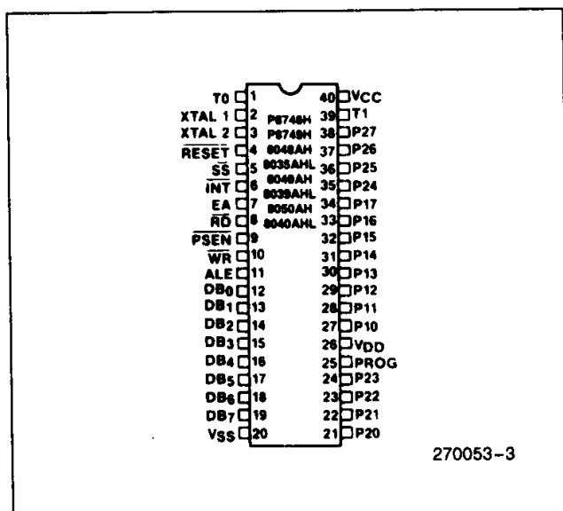
Figure 3. Pin Configuration
