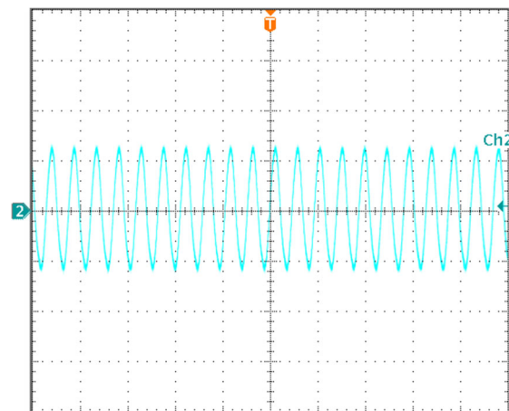
Figure 11: Output Voltage Ripple and Noise at nominal input voltage and max load current (20 mV/div, 2us/div) Load cap: 330\mu\text{F} , 50% ceramic, 50% Oscon. Bandwidth: 20MHz.
