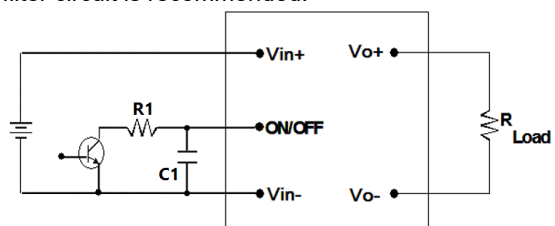
Figure 13: Remote On/Off Implementation
