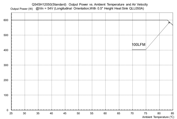
Figure 19: Output Power vs. Ambient Temperature and Air Velocity @Vin = 54V (Longitudinal Orientation, Airflow from Vout to Vin, With 0.5 inch Height Heat Sink QLL050A)
