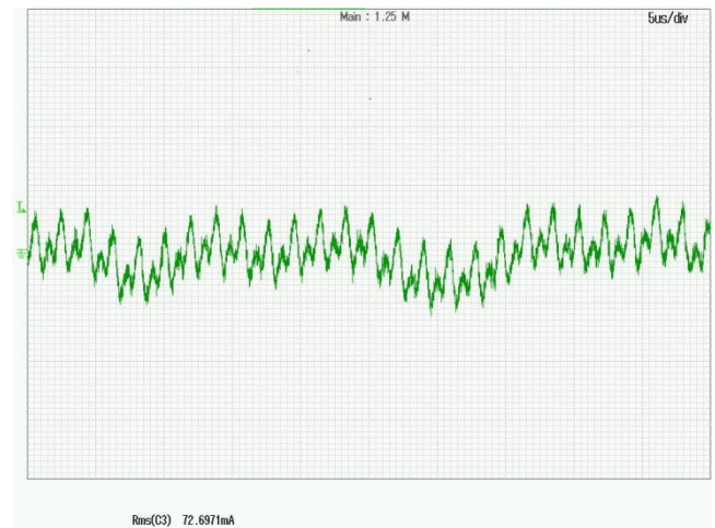
Figure 9: Input Terminal Ripple Current, i_c , at max output current and nominal input voltage with 12\mu\text{H} source impedance and 33\mu\text{F} electrolytic capacitor (200 mA/div, 5us/div).
