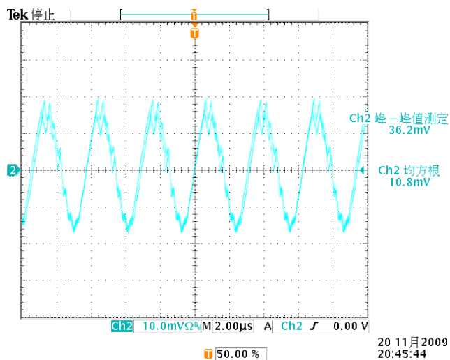
Figure 14: Output voltage ripple at nominal input voltage and rated load current ( I_o=25\text{A} ) (10 mV/div, 2us/div) Load capacitance: 1\mu\text{F} ceramic capacitor and 10\mu\text{F} tantalum capacitor. Bandwidth: 20 MHz.
