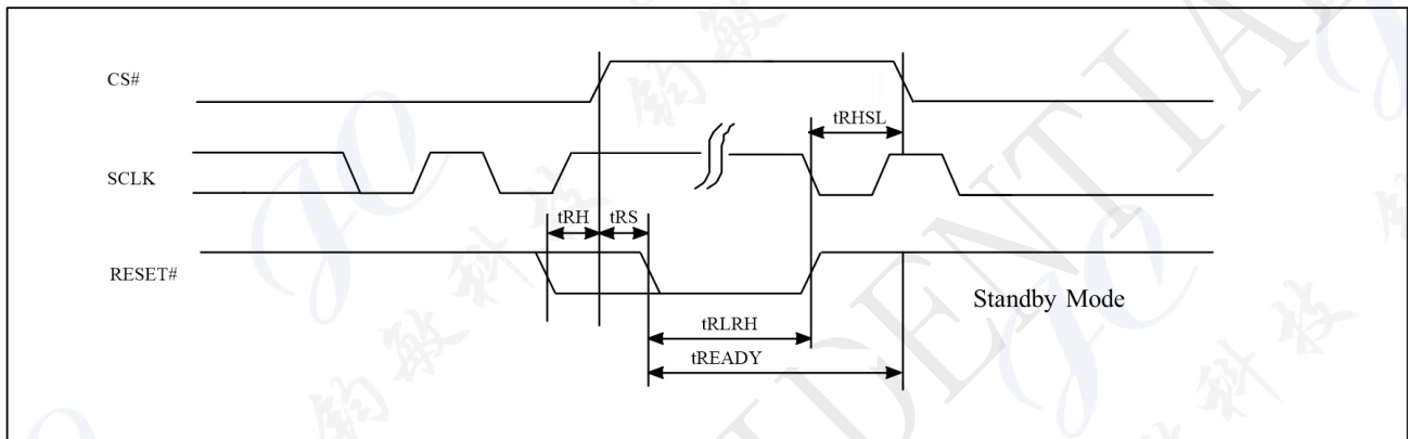
Figure 10-51 RESET Timing
