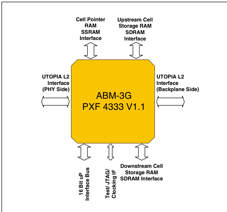
Figure 1-1 Logic Symbol
