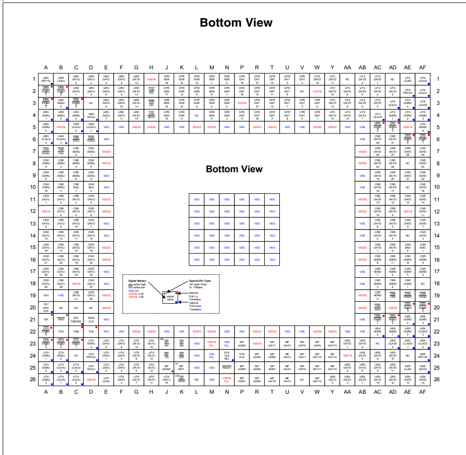
Figure 2-1 Pin Configuration (Bottom View)
