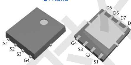
DFN5x6
