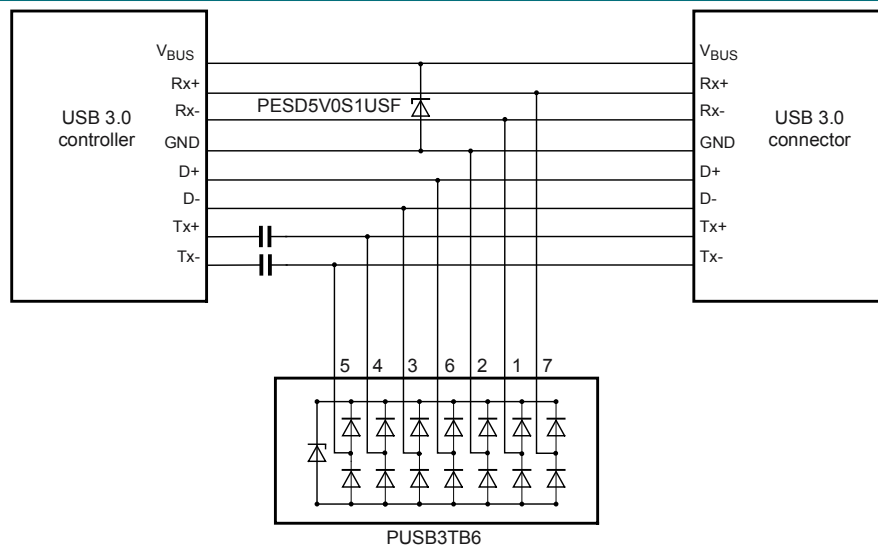
Fig. 10. Demo PCB of ESD protection for USB 3.0 or USB 2.0 interfaces using PUSB3TB6
