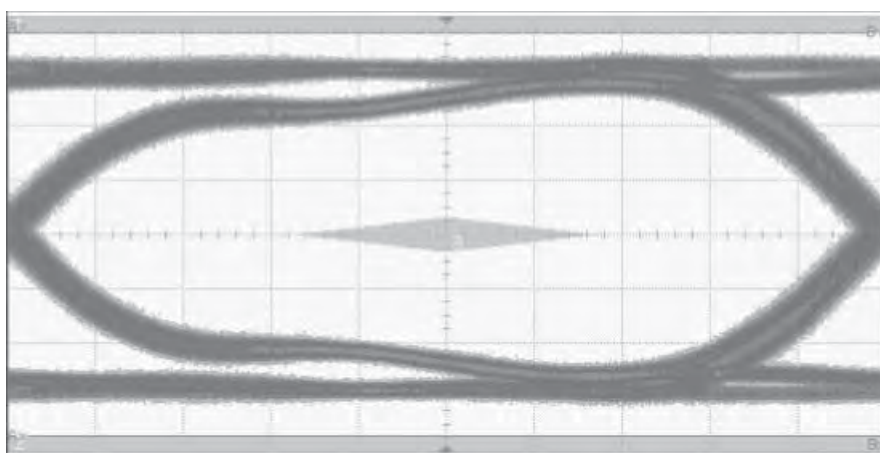
Fig 4. USB 3.0 eye diagram Printed-Circuit Board (PCB) with PUSB3TB6
