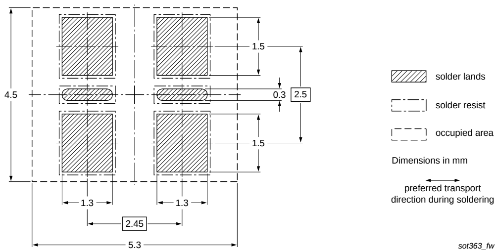
Fig 14. Wave soldering footprint PUMH11 (SOT363/SC-88)
