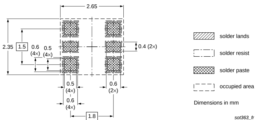
Fig 13. Reflow soldering footprint PUMH11 (SOT363/SC-88)
