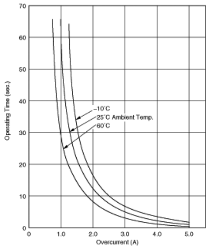
Operating Time (Typical Curve)
