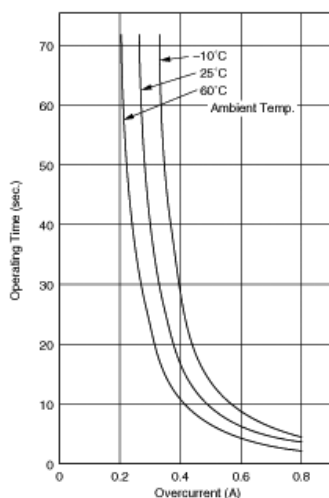
Operating Time (Typical Curve)
