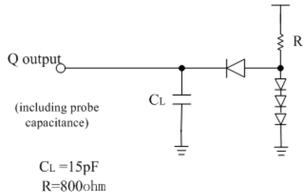
Load cct 2
