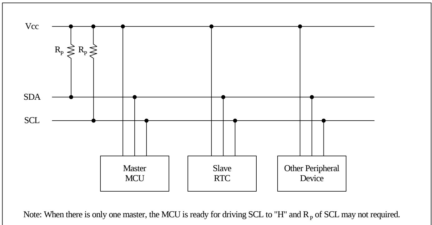
Fig.4 System configuration
