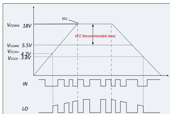
FIG. 1 VCC supply UVLO operating area
