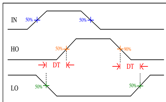
FIG. 3 Dead time protection
