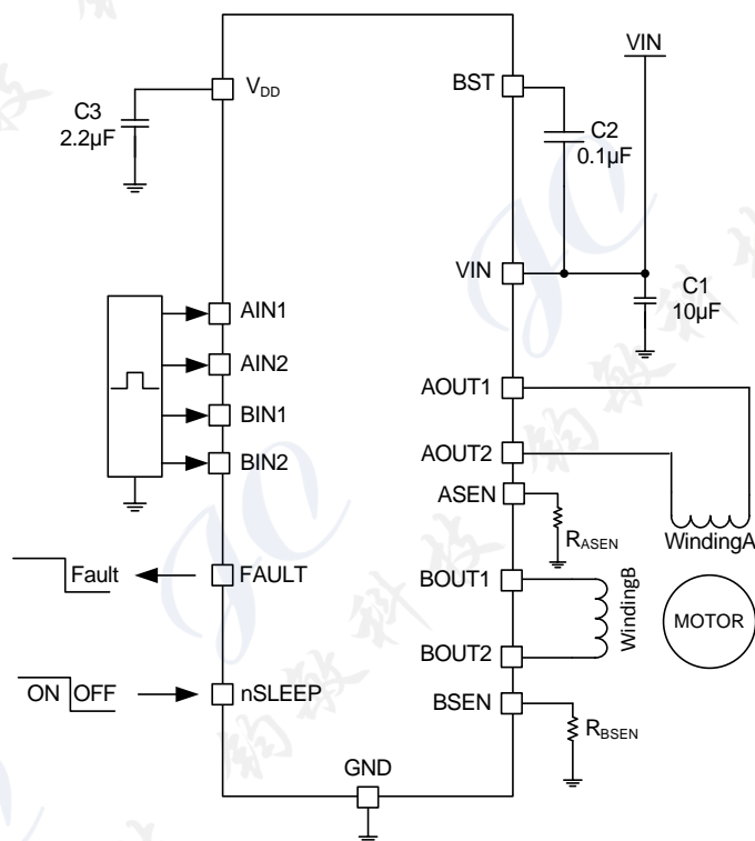
Stepper Motor Application
