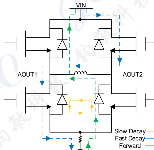
Figure 3: Reverse Operation
