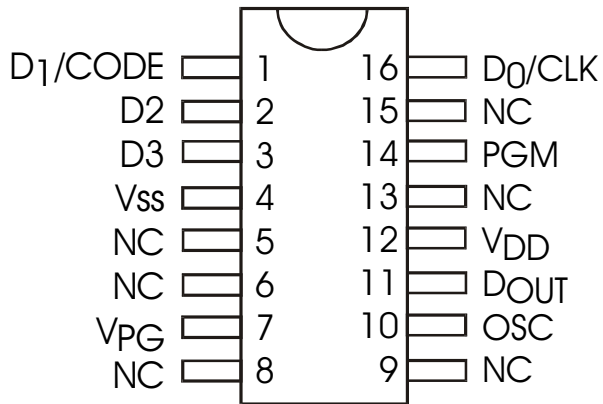
PT2282 (16 PINS)
