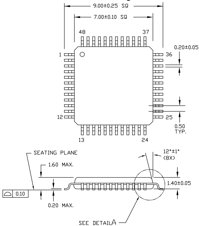
Figure 9. 48-Pin 7 × 7 × 1.4 mm TQFP Package Outline
