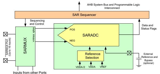
Figure 4. SAR ADC
