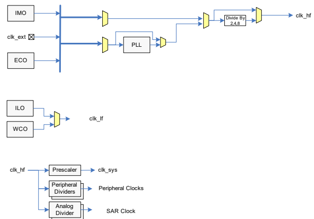
Figure 3. MCU Clocking Architecture
