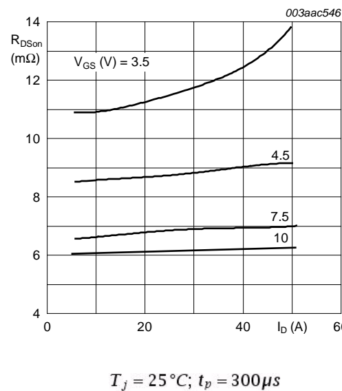
Fig 8. Drain-source on-state resistance as a function of drain current; typical values
