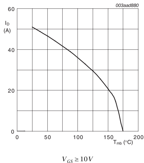
Fig 4. Continuous drain current as a function of mounting base temperature
