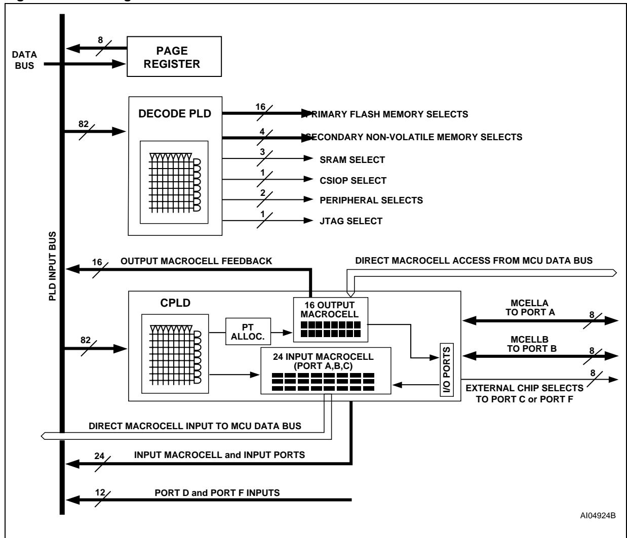
Figure 12. PLD Diagram
