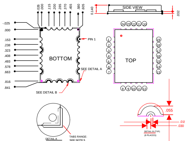
PHYSICAL DIMENSIONS
