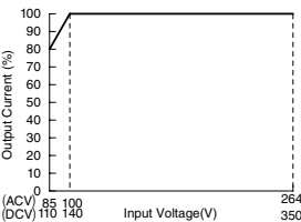
Overcurrent Protection Characteristics PS9Z-6RM*
