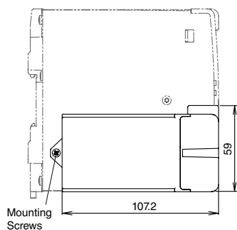
When using a PS9Z-6RM* DC-DC Converter Unit
