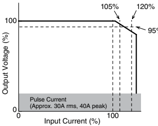
Overcurrent Protection Characteristics PS6R-J24
