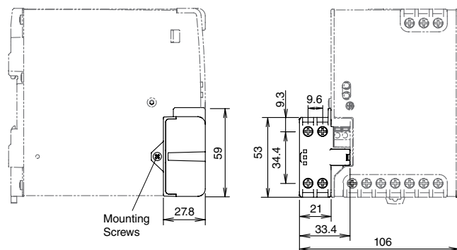
When using a PS9Z-6RS1 Branch Terminal Unit
