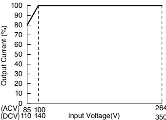
Output Current vs. Input Voltage (Derating Curves) PS9Z-J24 (Ta=25°C)
