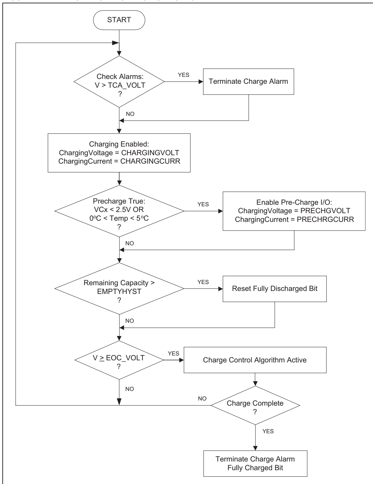
FIGURE 4-1: CHARGE INCREASING FLOW CHART
