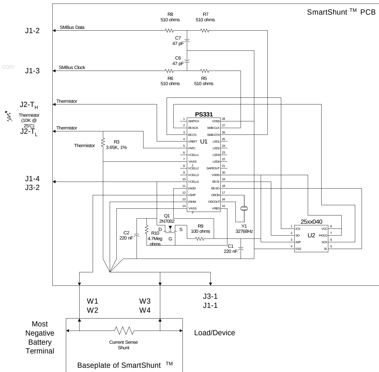
Figure 1. Electrical schematic of PS3180.
