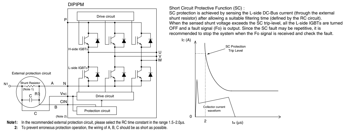
Fig. 6 EXTERNAL PART OF THE DIIPM PROTECTION CIRCUIT
