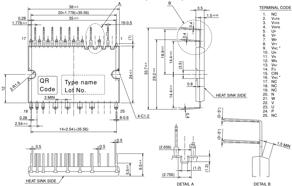
Fig. 3 ZIGZAG TERMINAL TYPE PACKAGE OUTLINES (PS21962-CT)
