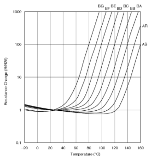
Resistance-Temperature Characteristics
