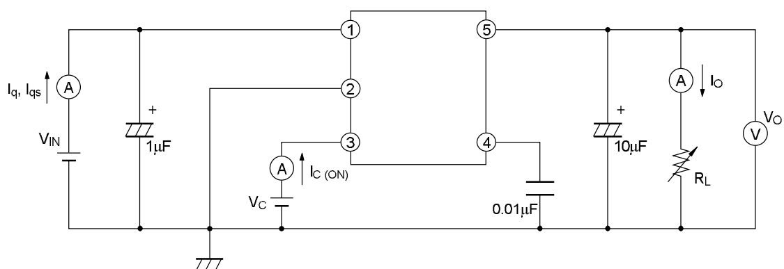
Fig.1 Test Circuit
