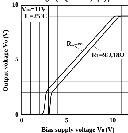
Fig.9 Output Voltage vs. Bias Supply Voltage (PQ09NF1) (Typical value)
