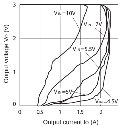
Fig.8 Overcurrent Protection Characteristics (PQ033EZ1HZxH)
