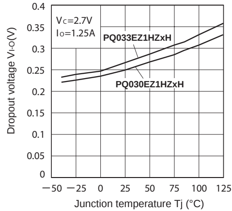
Fig.24 Dropout Voltage vs. Junction Temperature
