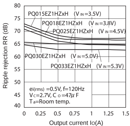
Fig.27 Ripple Rejection vs. Output Current
