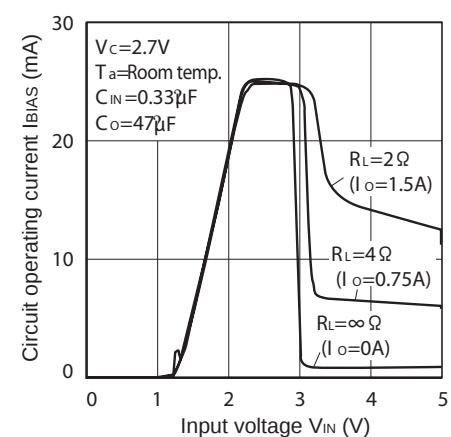
Fig.22 Circuit Operating Current vs. Input Voltage (PQ030EZ1HZxH)
