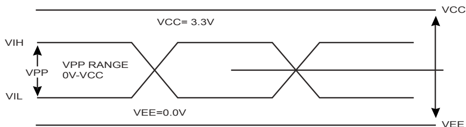
FIGURE 2. HSTL/HSTL OUTPUT
