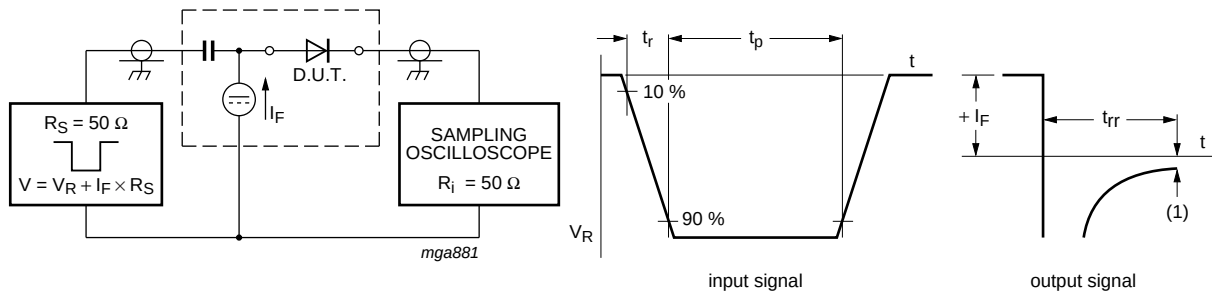
Fig 14. Reverse recovery time: test circuit and waveforms
