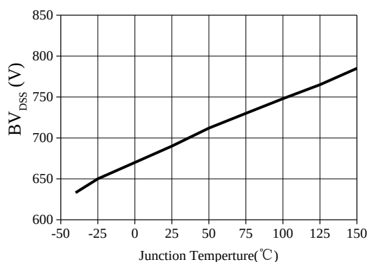
(c) BV_{DS} vs T_j
