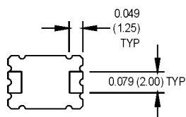
SUGGESTED SOLDER PAD LAYOUT
