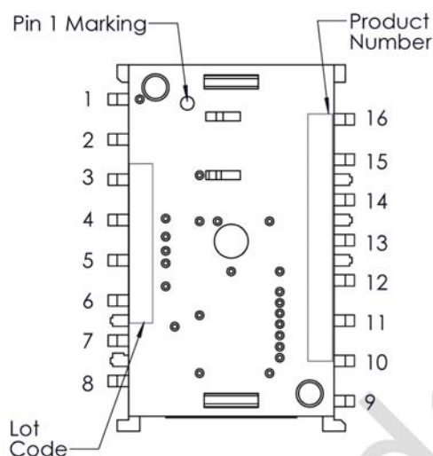
Figure 2. Device Pinout
