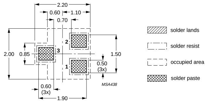
Fig 15. Reflow soldering footprint for SOT416 (SC-75).
