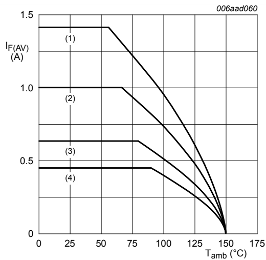
FR4 PCB, mounting pad for cathode 1 cm 2 T_j = 150 °C (1) \delta = 1 (2) \delta = 0.5 (3) \delta = 0.2 (4) \delta = 0.1
