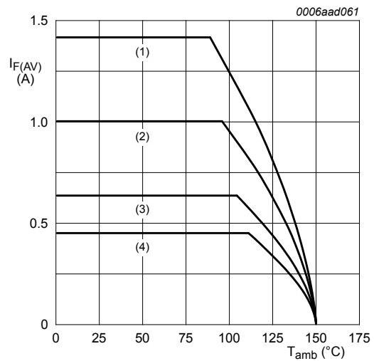
Ceramic PCB, Al 2 O 3 , standard footprint T_j = 150 °C (1) \delta = 1 (2) \delta = 0.5 (3) \delta = 0.2 (4) \delta = 0.1
