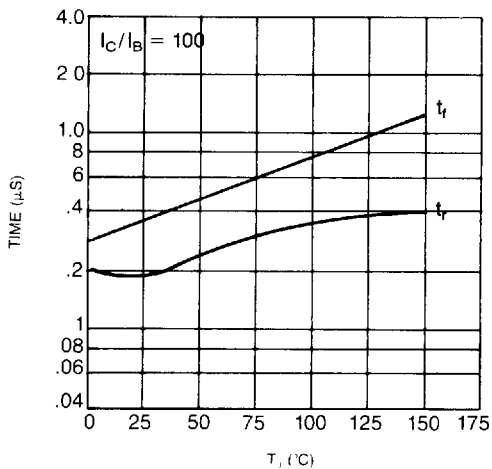
DYNAMIC CHARACTERISTICS VS JUNCTION TEMPERATURE
