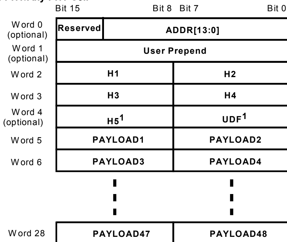
Fig. 3 SCI-PHY/Any-PHY Cell
