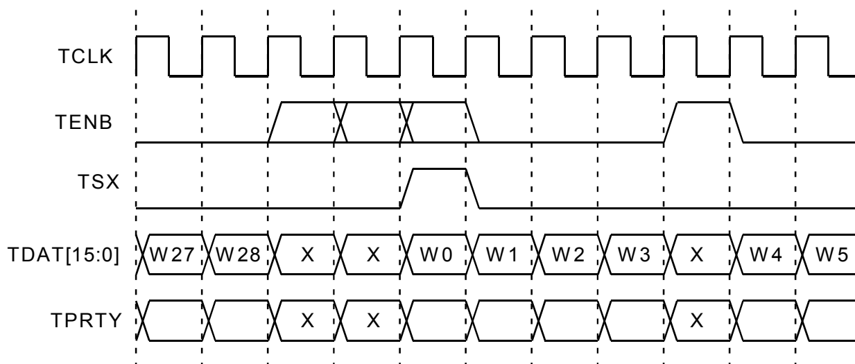
Fig. 13 Downstream Any-PHY Interface Transfer Timing
