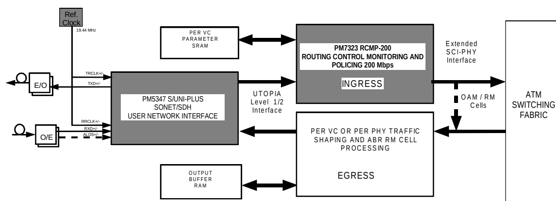
Figure 1 - OC-3 Switch Port Application
