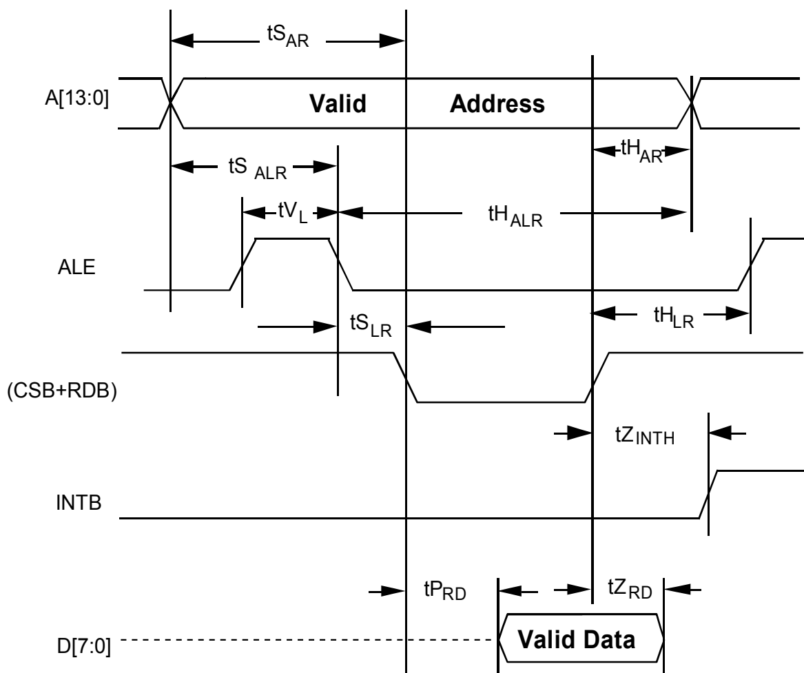
Figure 30 - Microprocessor Interface Read Access Timing (Intel Mode)
