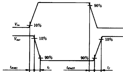
WAVEFORMS
