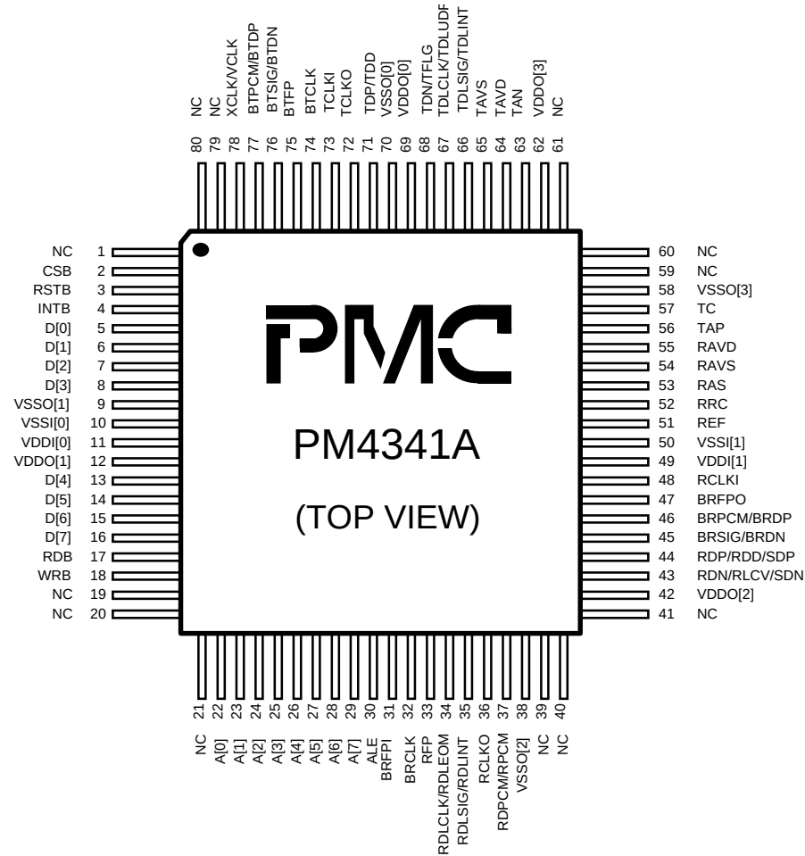
Figure 5 - 80 Pin PQFP
