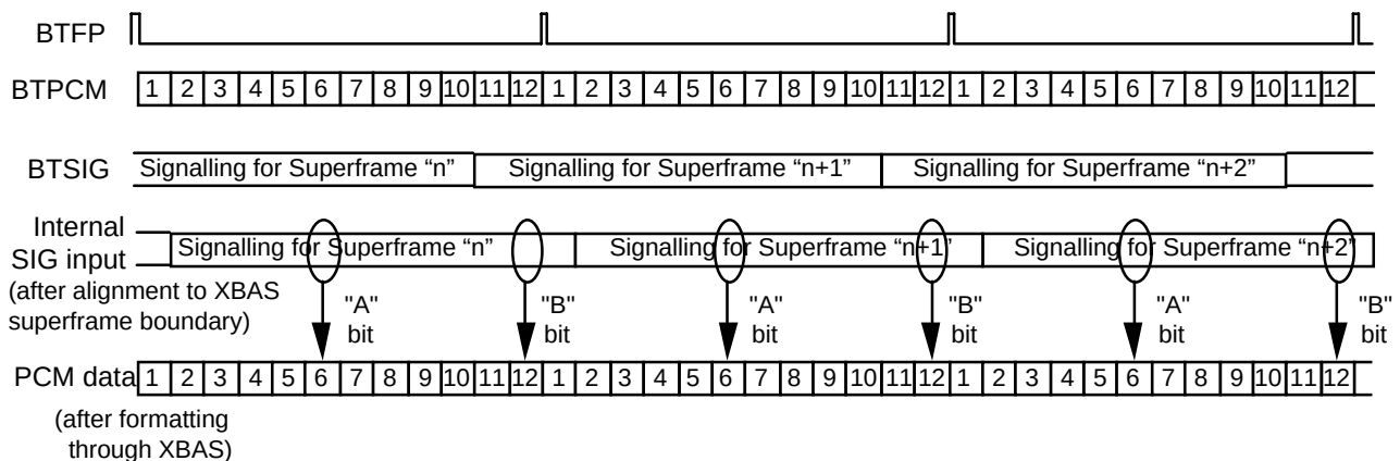
Figure 31 - 1.544MHz Transmit Backplane Interface - with signalling alignment
