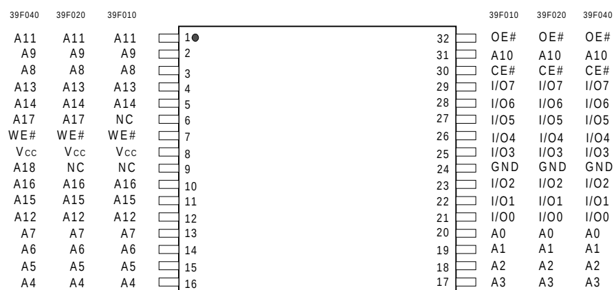
32-Pin VSOP
