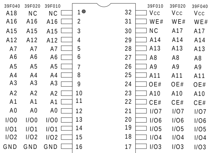
32-Pin PDIP
