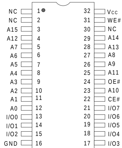
32-Pin PDIP
