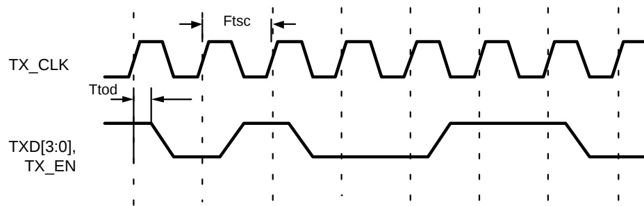
MII Interface Transmit Signals
