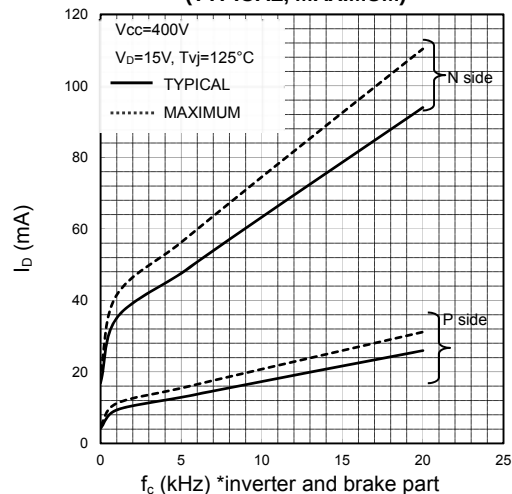
I_D VS. f_c CHARACTERISTICS (TYPICAL, MAXIMUM)
