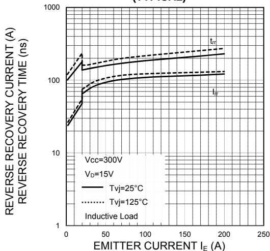
FREE WHEELING DIODE REVERSE RECOVERY CHARACTERISTICS (TYPICAL)
