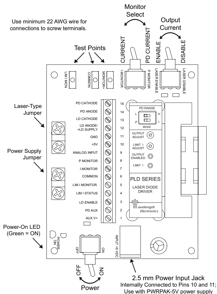
Figure 7. PLDEVALPCB Evaluation Board
