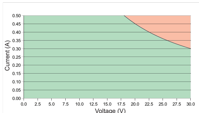
Figure 24. SOA for PLD500
