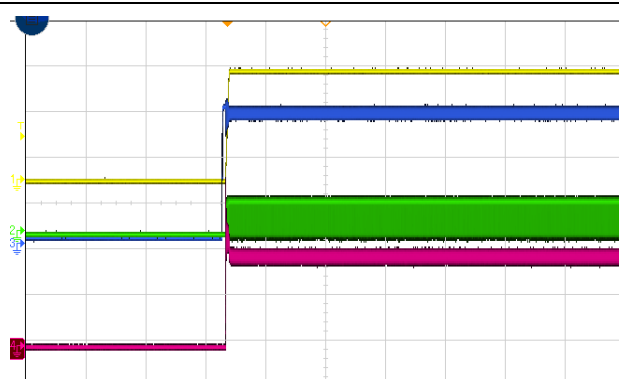
Fig. 6 Power Up Waveform, Iout=2A
