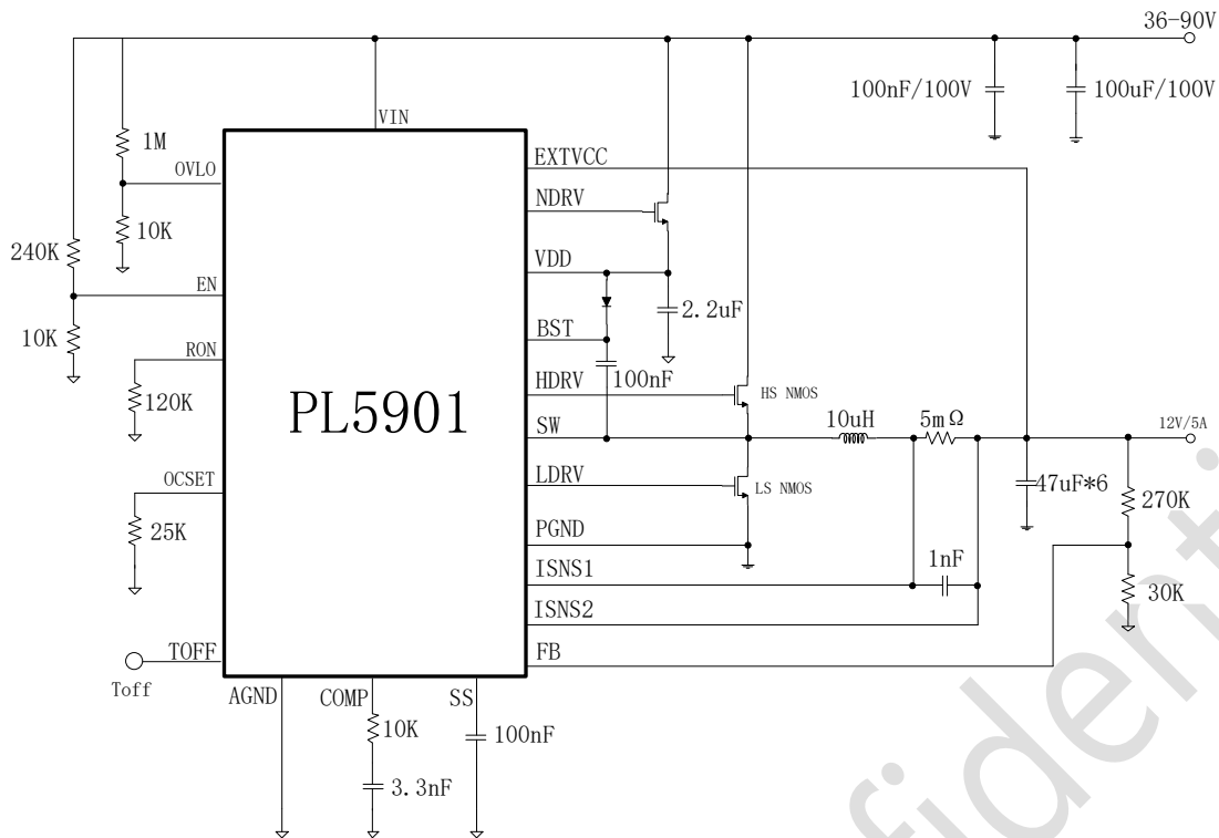
Figure 23. Application Schematic
