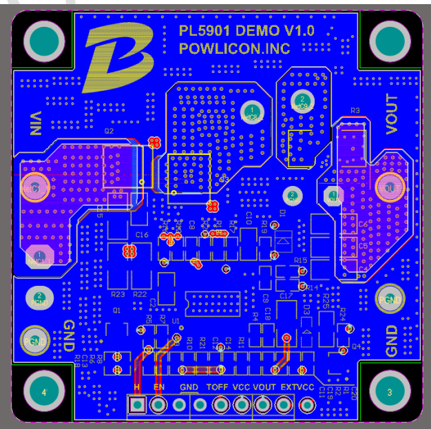
Figure 25. Bottom lay
