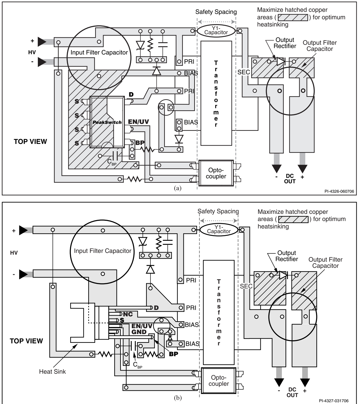
Figure 17. Recommended Layout for PeakSwitch in (a) P and (b) Y/F Packages.
